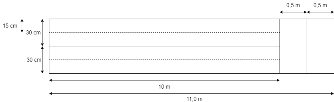
Figure 4: Approximate dimensions of the race track.
